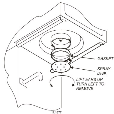
Fig. 12 Cleaning
