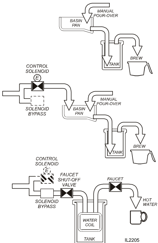
Fig. 5 Heat Control Diagram
