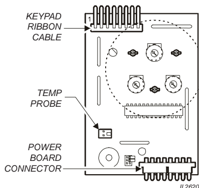
Fig. 18 Controller Hook-Up
